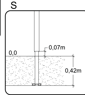
S Sunken Foundation 8112801
